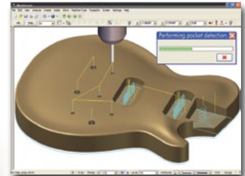
Mastercam's Feature Based Machining (FBM) automates the programming of 2D solid features.
