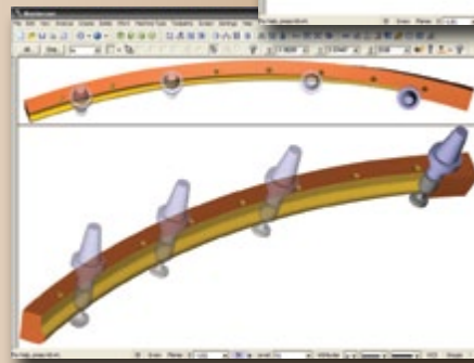
Multisurface swarf cutting keeps the tool edge against the surface for a smooth finish.
