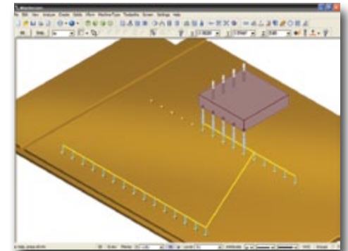
Fully optimized drilling, including block drilling.
